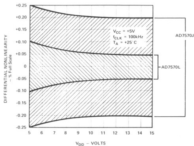
Figure 3. Differential Nonlinearity vs. V_{DD}
