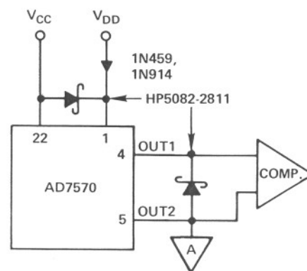
Figure 12. Diode Protection Scheme
