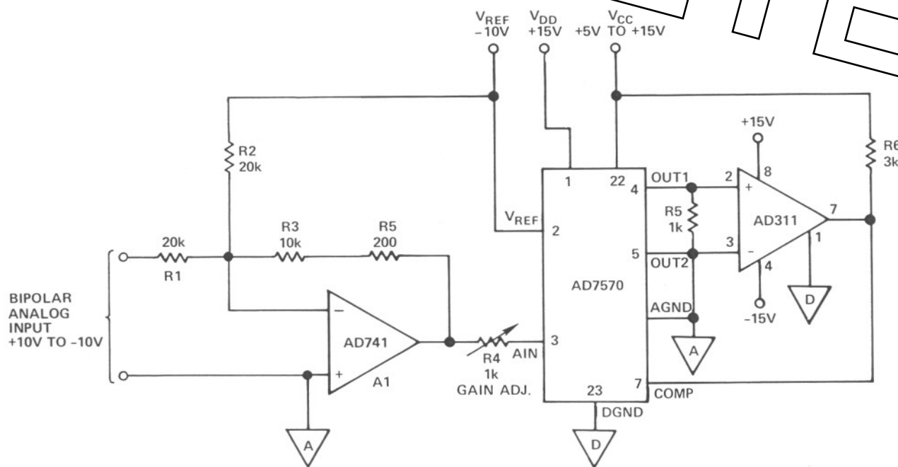
Figure 10. Unipolar Operation
