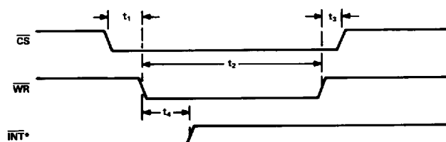
Figure 1. AD7579/AD7580 Start Cycle Timing
