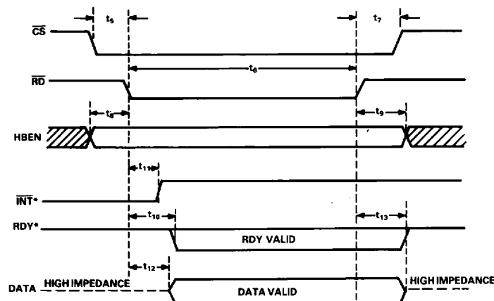
Figure 2. AD7579/AD7580 Read Cycle Timing
