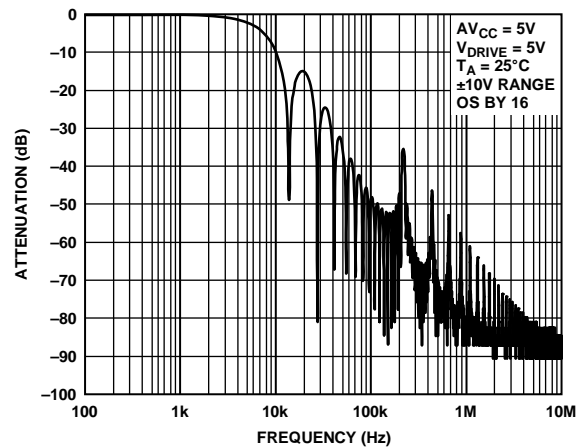
Figure 56. Digital Filter Response for OS × 16
