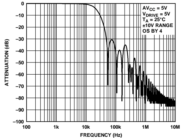
Figure 54. Digital Filter Response for OS × 4
