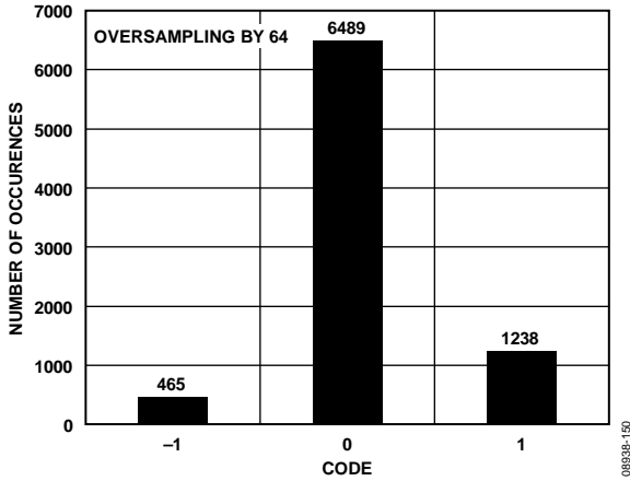
Figure 52. Histogram of Codes—OS × 64 (3 Codes)
