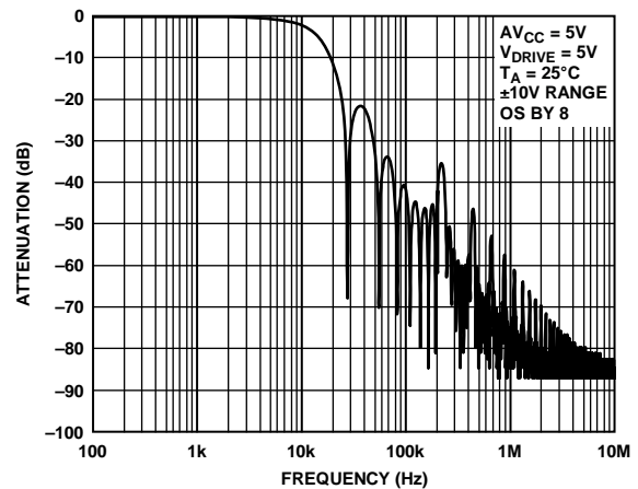
Figure 55. Digital Filter Response for OS × 8
