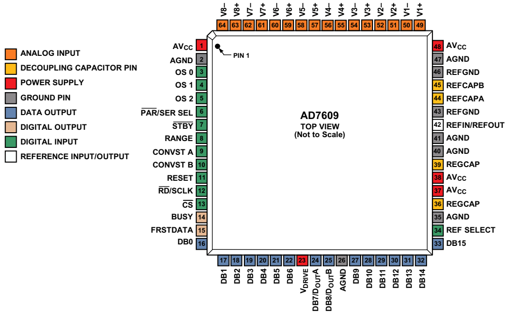
Figure 7. Pin Configuration
