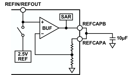
Figure 38. Reference Circuitry
