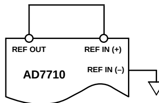
Figure 8. REF OUT/REF IN Connection
