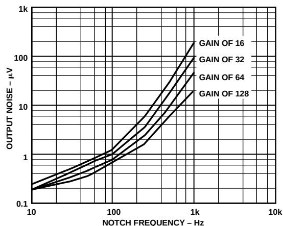
Figure 2b. Plot of Output Noise vs. Gain and Notch Frequency (Gains of 16 to 128)
