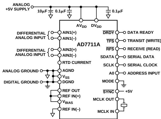
Figure 3. Basic Connection Diagram
