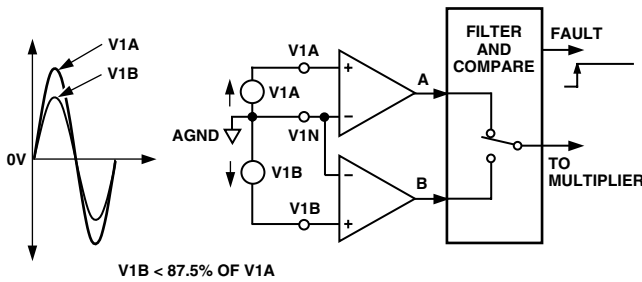
Figure 13. Fault Conditions for Inactive Input Less than Active Input
