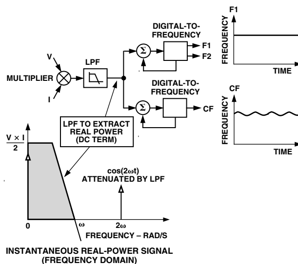
Figure 12. Real-Power-to-Frequency Conversion
