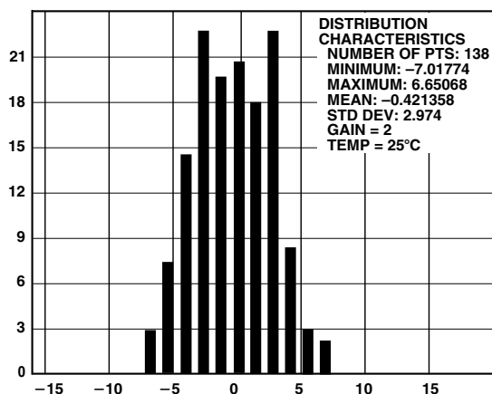
TPC 13. Channel 1 Offset Distribution (Gain = 2)
