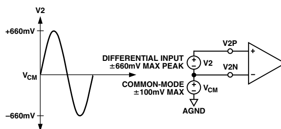
Figure 23. Maximum Signal Levels, Channel 2
