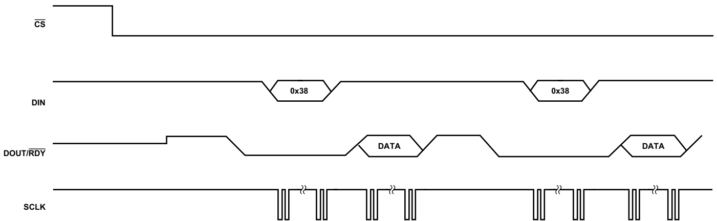
Figure 9. Continuous Conversion
