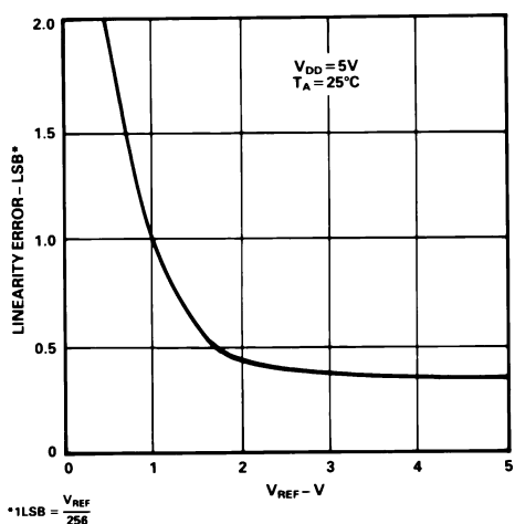
TPC 2. Accuracy vs. V_{REF} [ V_{REF} = V_{REF(+)} - V_{REF(-)} ]
