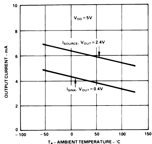
TPC 6. Output Current vs. Temperature
