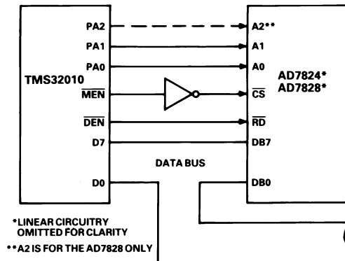
Figure 18. AD7824/AD7828–TMS32010 Interface
