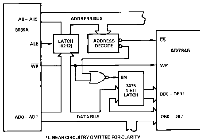
Figure 22. 8085A Interface
