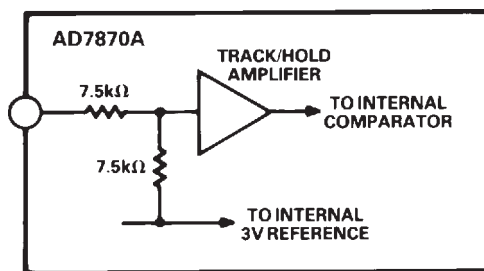
Figure 4. Analog Input
