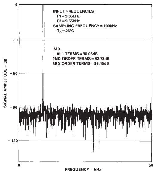
Figure 15. IMD Plot
