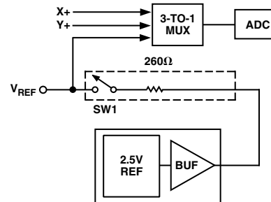
Figure 5. On-Chip Reference Circuitry
