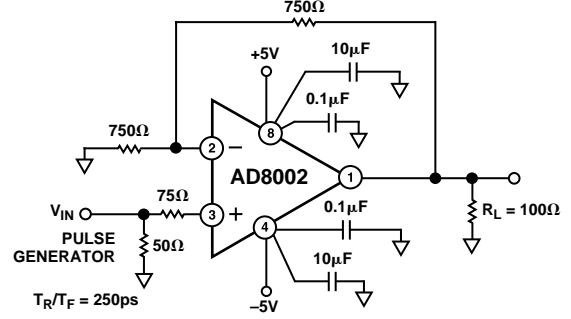
Figure 7. Test Circuit, Gain = +2
