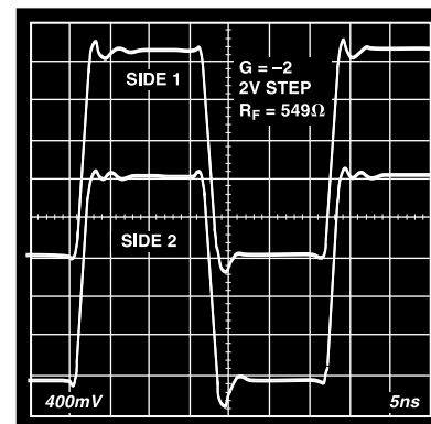
Figure 38. 2 V Step Response, G = -2
