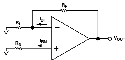
Figure 5. Output Offset Voltage
