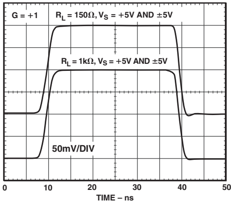
TPC 37. Small Signal Transient Response for R_L = 150\ \Omega , 1\ \text{k}\Omega and V_S = +5\ \text{V} , \pm 5\ \text{V}
