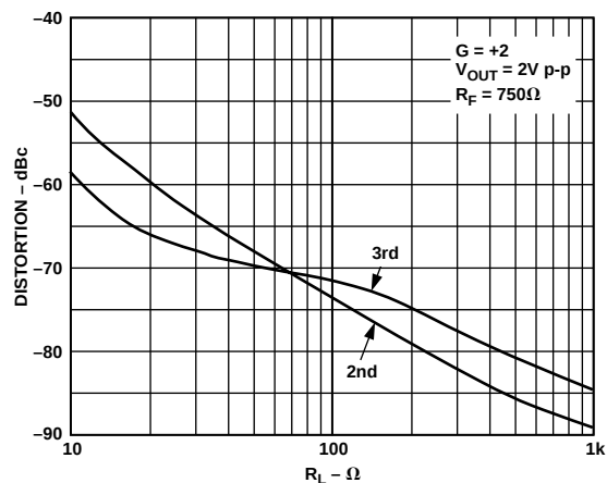
Figure 16. Distortion vs. Load Resistance; V_S = \pm 5\text{ V} , Frequency = 500 kHz
