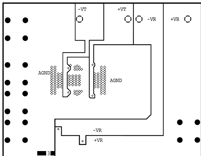
Figure 49. Power/Ground Plane
