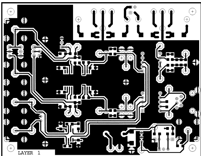
Figure 48. Layer 1
