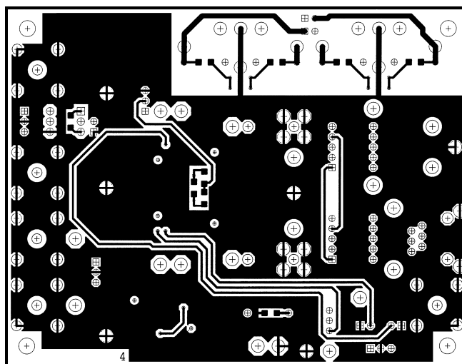
Figure 50. Layer 1
