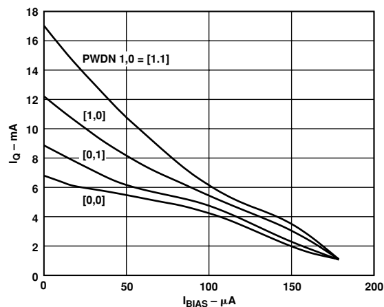
Figure 35. I_Q vs. I_{BIAS} Pin Current; V_S = \pm 6\text{ V}
