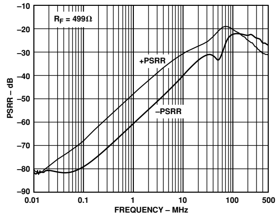
Figure 26. PSRR vs. Frequency; V_S = \pm 12\text{ V}
