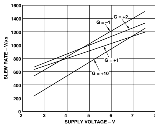
Figure 22. Maximum Slew Rate vs. Supply Voltage
