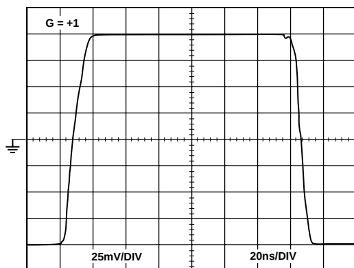
TPC 19. Small Signal Transient Response +5\text{ V} (See Test Circuit 1)
