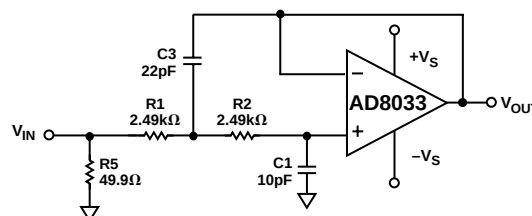
Figure 10. Two-Pole Butterworth Active Filter
