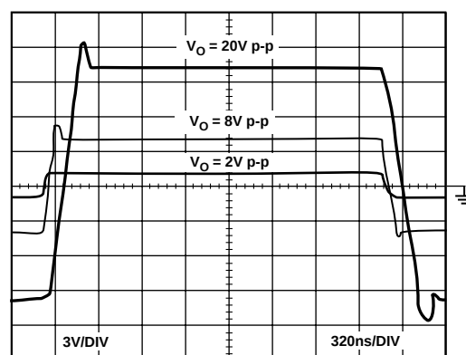
TPC 23. Large Signal Transient Response G = +2 (See Test Circuit 2)
