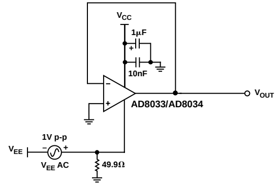
Test Circuit 8. Negative PSRR
