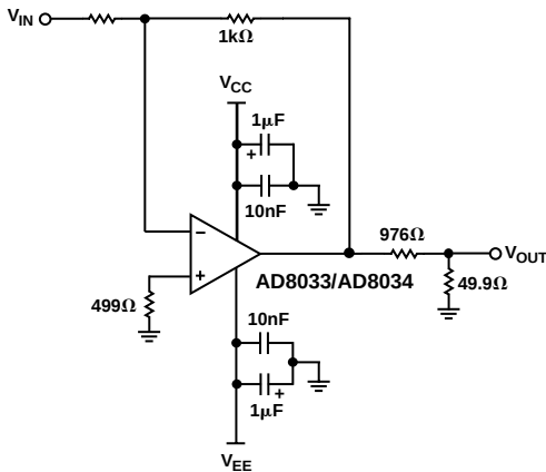
Test Circuit 3. G = -1
