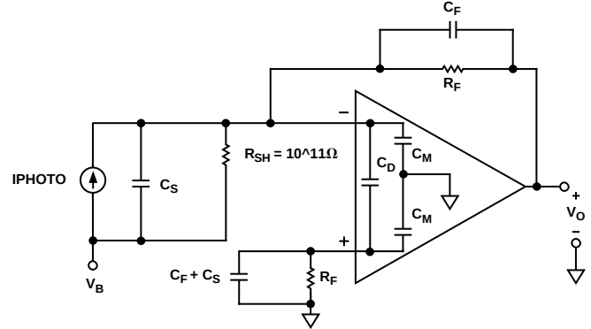
Figure 12. Wideband Photodiode Preamplifier
