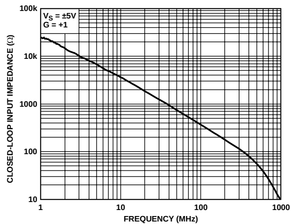
Figure 48. Input Impedance vs. Frequency
