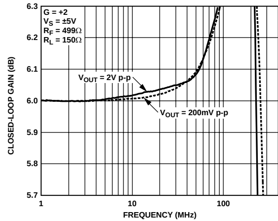
Figure 12. 0.1 dB Flatness vs. Frequency for Various Output Voltages
