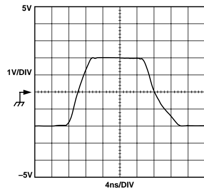
Figure 14. Large Signal Step Response G = +1 , R_L = 1 \text{ k}\Omega , V_S = \pm 5.0 \text{ V}
