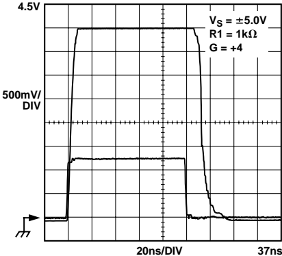
Figure 31. Output Overload Recovery, V_S = \pm 5.0\text{ V}
