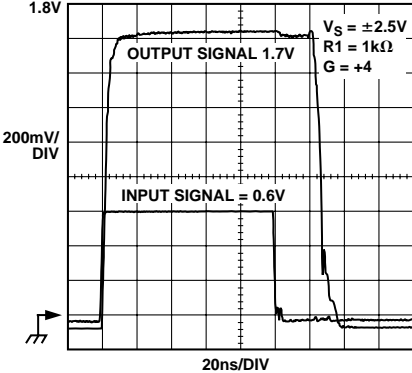
Figure 30. Output Overload Recovery, V_S = \pm 2.5\text{ V}
