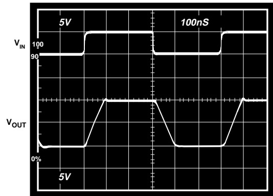
Figure 46. AD810 Driving a 1000 pF Load, Gain = +2, R_F = 750 \Omega , R_S = 11 \Omega , R_L = 10 k\Omega
