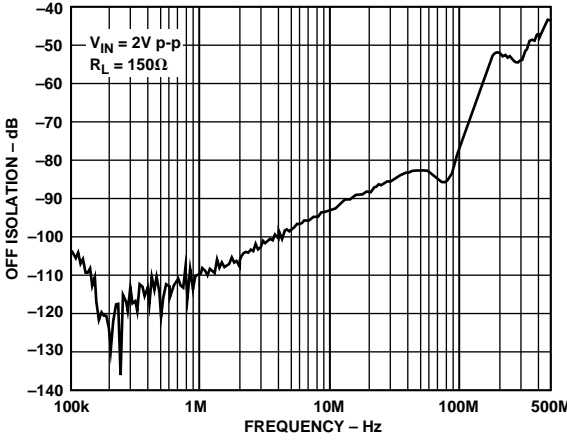
Figure 22. AD8108 Off Isolation, Input-Output
