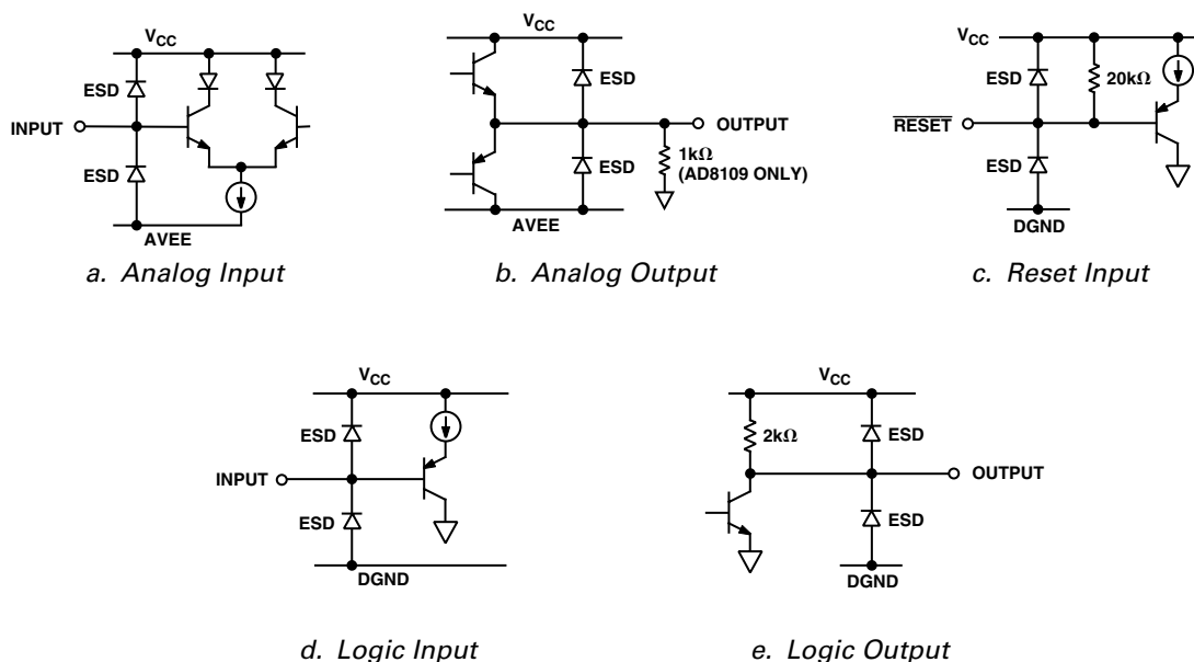
Figure 5. I/O Schematics
