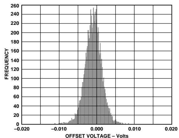
Figure 34. AD8110 Offset Voltage Distribution
