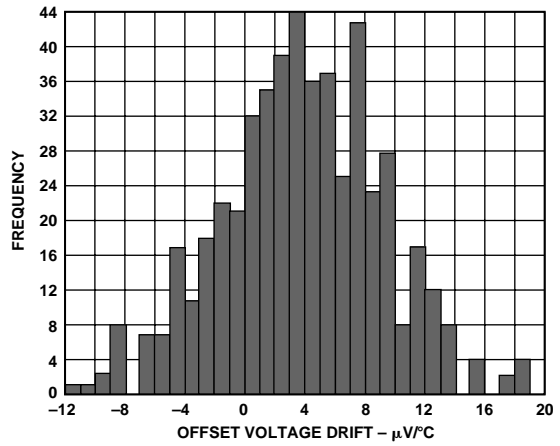
Figure 41. AD8115 Offset Voltage Drift Distribution (-40°C to +85°C)
