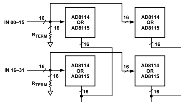
Figure 42. 32 \times 32 Crosspoint Array Using Four AD8114s or Four AD8115s
