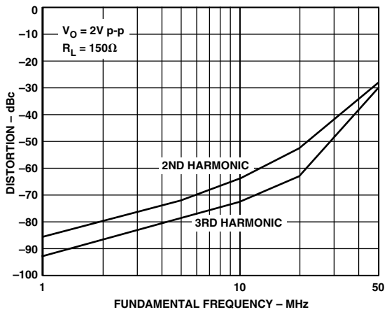
TPC 8. AD8114 Distortion vs. Frequency
