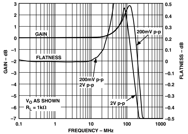
TPC 5. AD8115 Frequency Response; R_L = 1 \text{ k}\Omega
