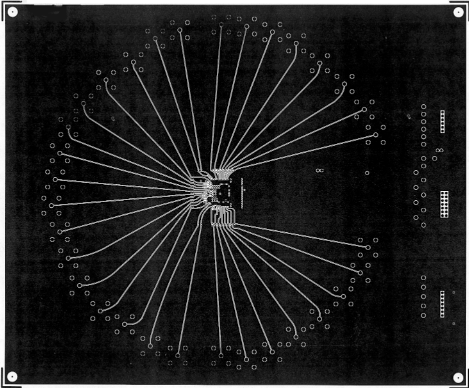
Figure 11. Board Layout (Signal Layer)
