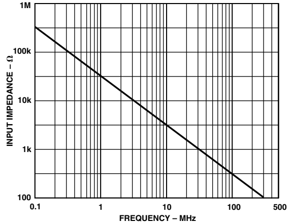
TPC 16. AD8115 Input Impedance vs. Frequency
