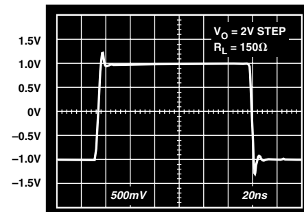
TPC 29. AD8115 Pulse Response, Large Signal
