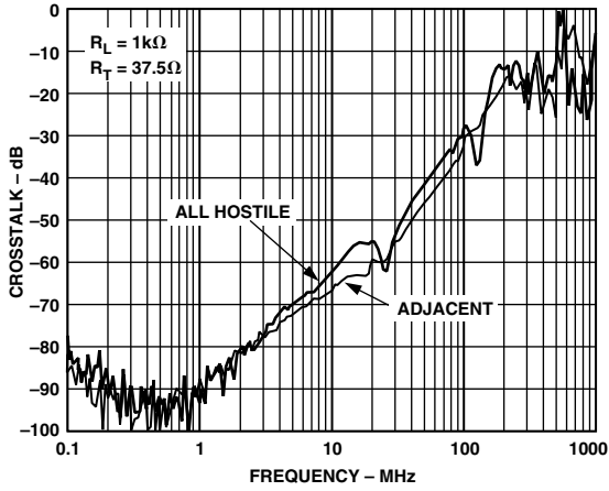
TPC 7. AD8114 Crosstalk vs. Frequency
