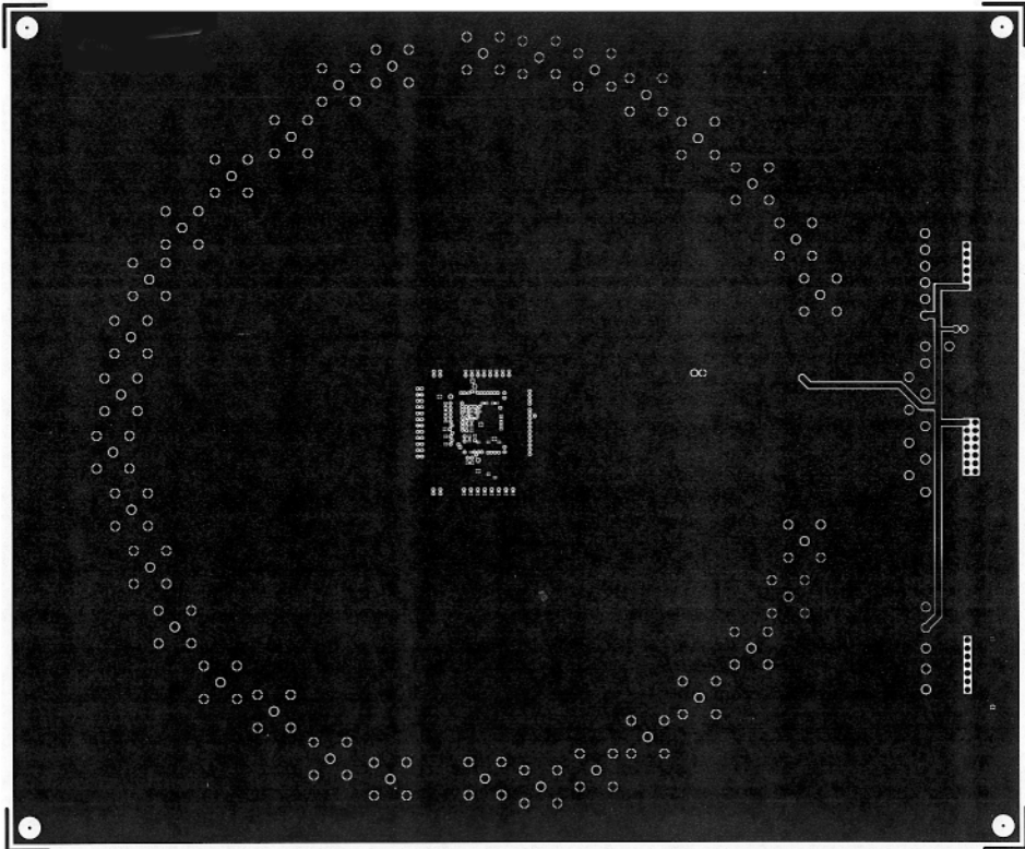
Figure 12. Board Layout (Ground Plane)
