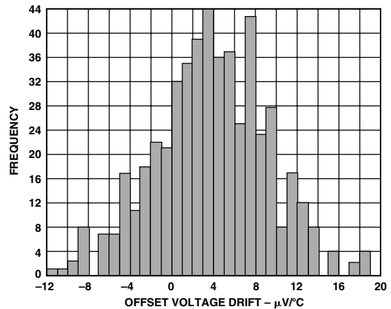
TPC 36. AD8115 Offset Voltage Drift Distribution (-40°C to +85°C)
