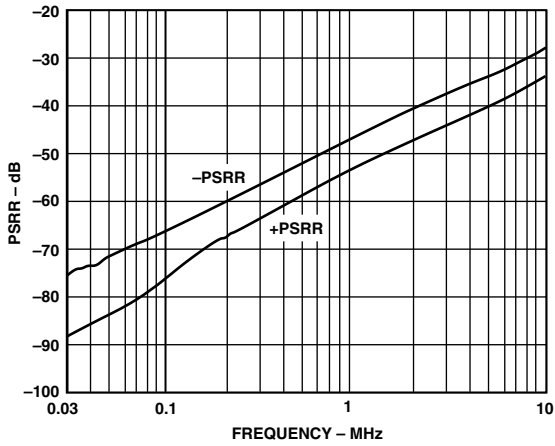
TPC 20. AD8114 PSRR vs. Frequency
