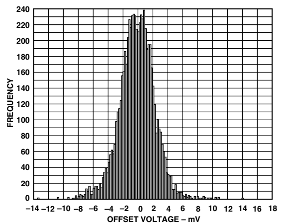
TPC 35. AD8115 Offset Voltage Distribution
