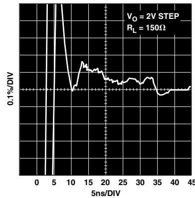
TPC 12. AD8115 Settling Time
