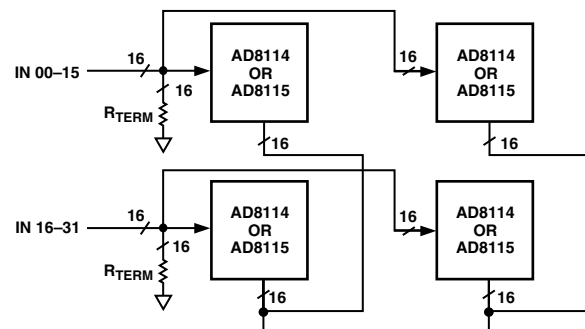
Figure 6. 32 \times 32 Crosspoint Array Using Four AD8114s or Four AD8115s
