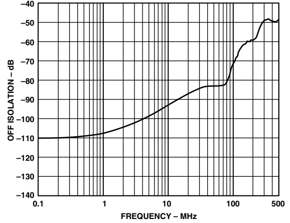
TPC 22. AD8115 Off Isolation, Input-Output
