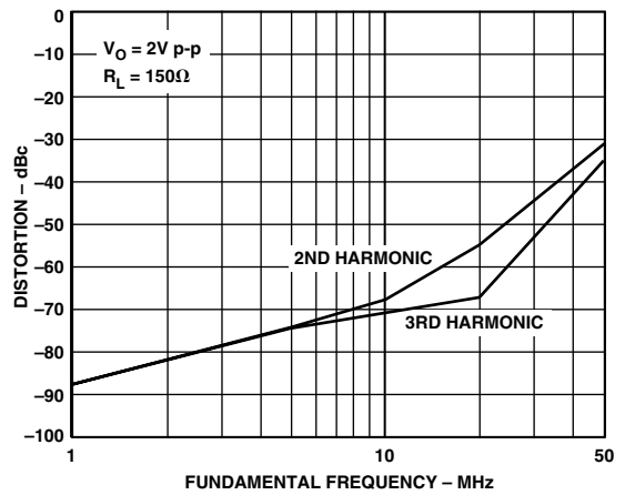
TPC 11. AD8115 Distortion vs. Frequency
