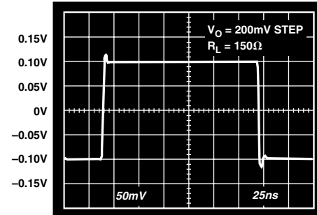
TPC 28. AD8115 Pulse Response, Small Signal
