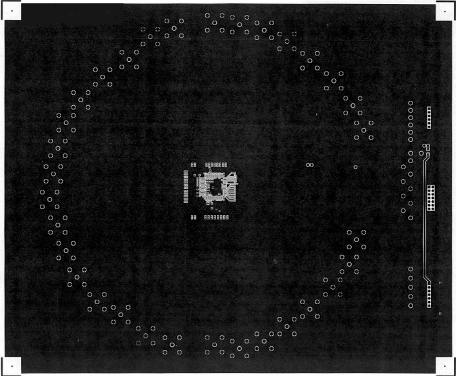
Figure 10. Board Layout (Component Side)
