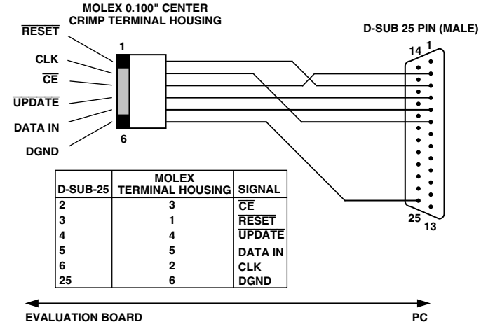
Figure 16. Evaluation Board-PC Connection Cable
