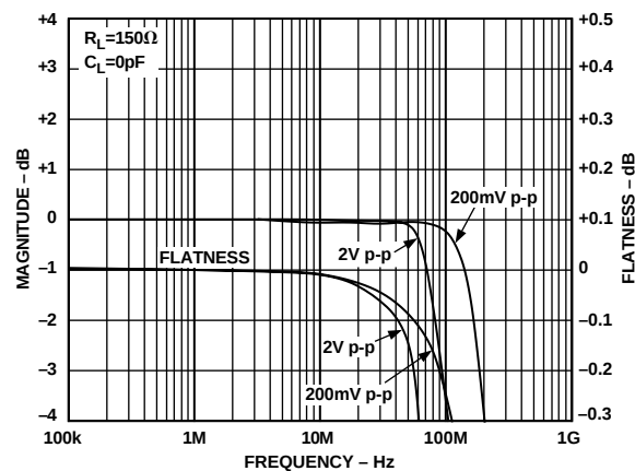
Figure 6. Frequency Response
