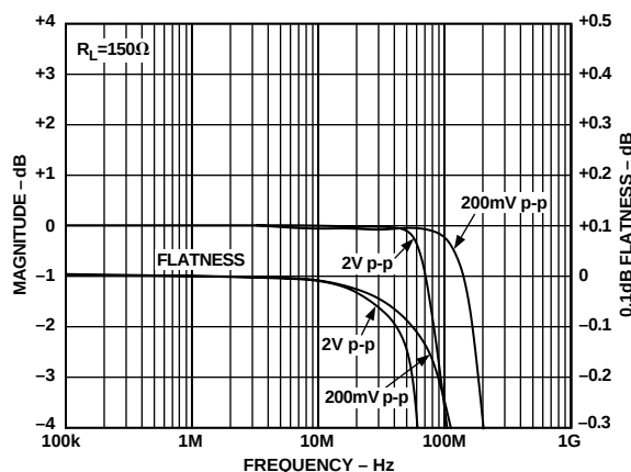
Figure 1. Frequency Response
