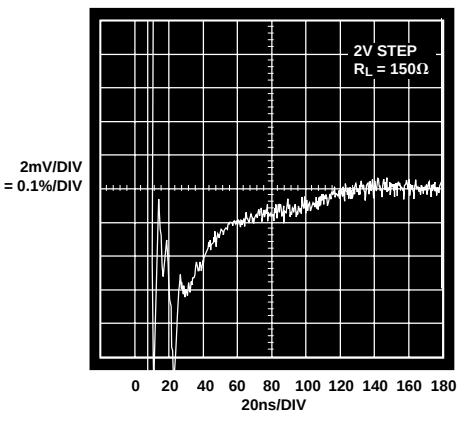
Figure 11. Settling Time
