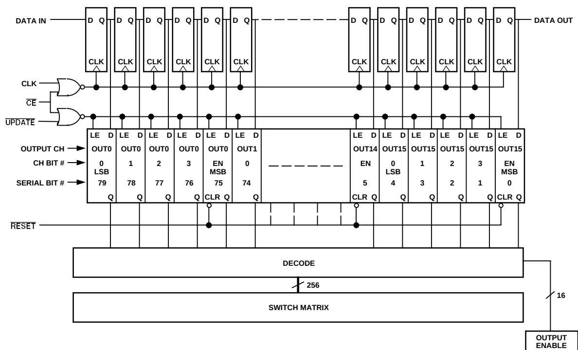
Figure 4. Logic Diagram
