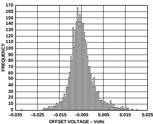
Figure 22. Offset Voltage Distribution
