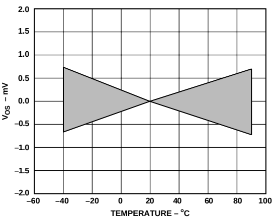
Figure 23. Offset Voltage Drift vs. Temperature
