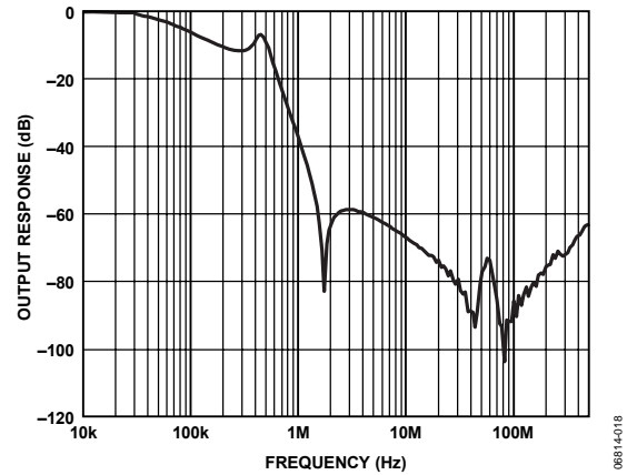
Figure 31. Power Supply Filter Frequency Response in a 50 Ω System
