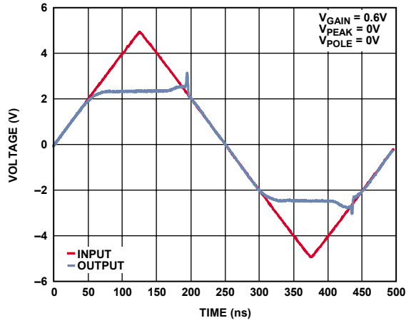
Figure 10. Overdrive Recovery
