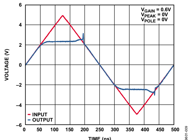
Figure 9. Overdrive Recovery
