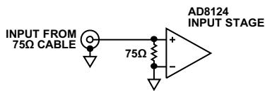
Figure 24. Terminating a 75 \Omega Cable
