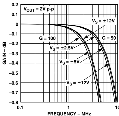
TPC 32. AD8129 Fine Scale Response vs. Supply, G = 50 , G = 100 , V_{OUT} = 2\text{ V p-p}
