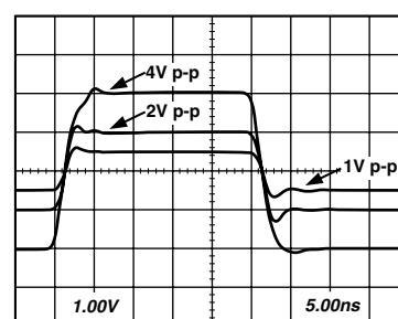
TPC 81. AD8130 Transient Response vs. Output Amplitude, V_{OUT} = 1\text{ V p-p} , 2\text{ V p-p} , 4\text{ V p-p}
