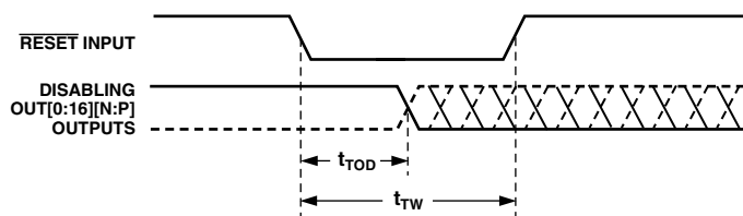
Figure 29. Asynchronous Reset
