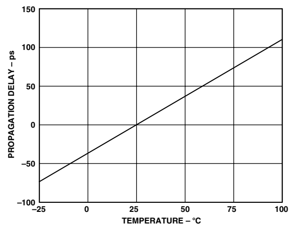
Figure 18. Propagation Delay, Normalized at 25°C vs. Temperature
