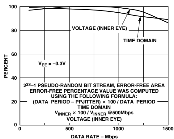
Figure 11. AC Performance
