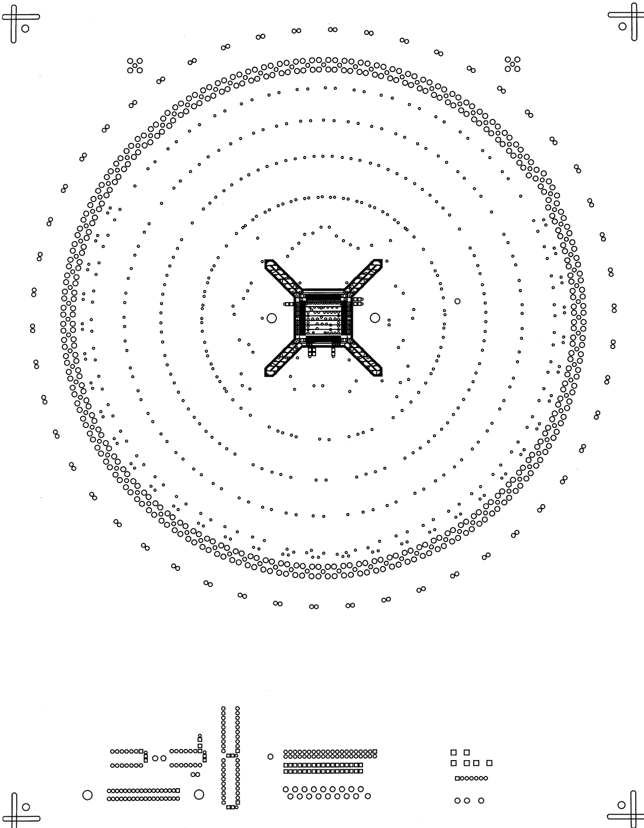
Figure 44. Soldermask Top
