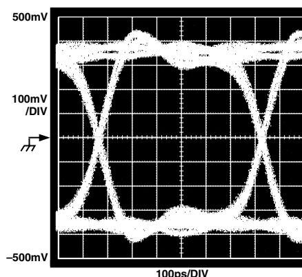
Figure 1. Output Eye Pattern, 1.5 Gbps
