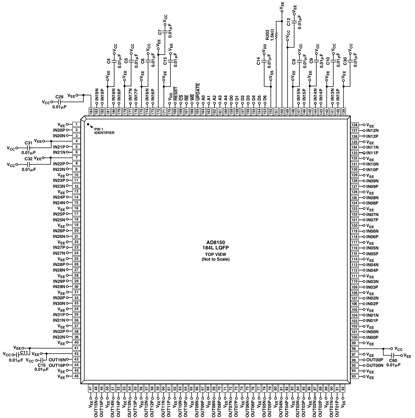
Figure 49. Bypassing Schematic
