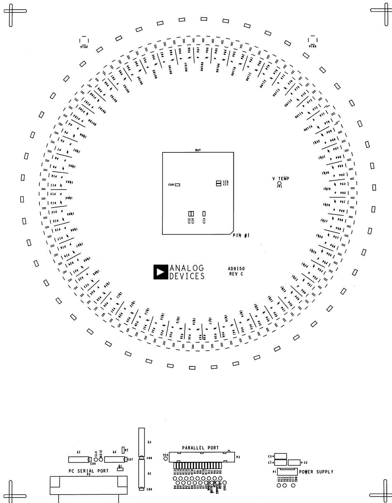
Figure 43. Silkscreen Top
