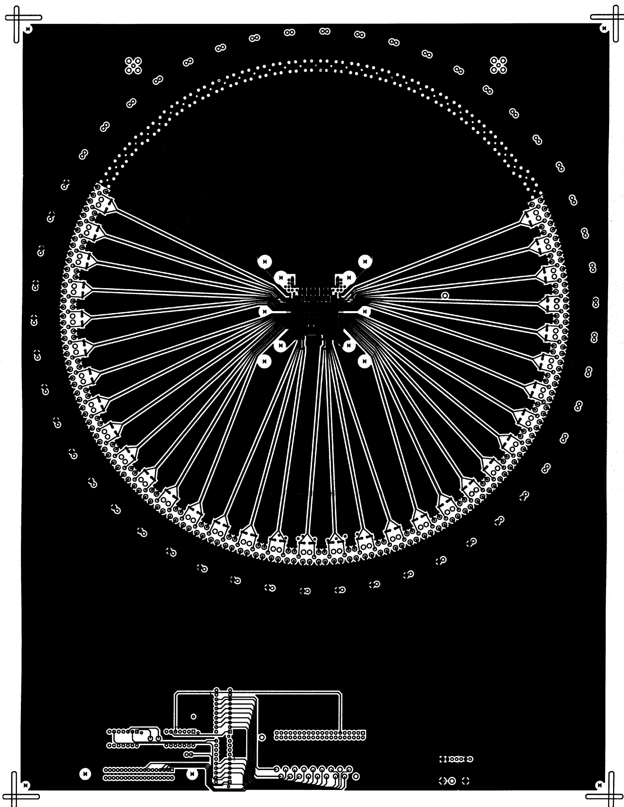
Figure 42. Circuit Side
