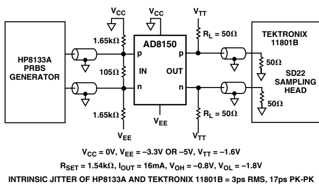
Figure 22. Eye Pattern Test Circuit
