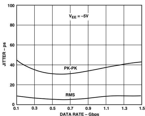
Figure 8. Jitter vs. Data Rate, PRBS 23
