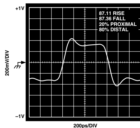
Figure 20. Rise/Fall Times, V_{EE} = -5 V
