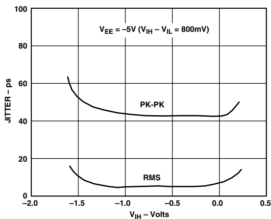
Figure 7. Jitter vs. V_{IH} 1.5 Gbps, PRBS 23
