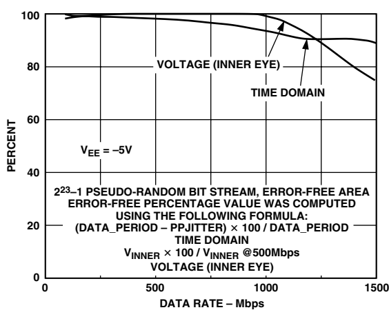
Figure 14. AC Performance
