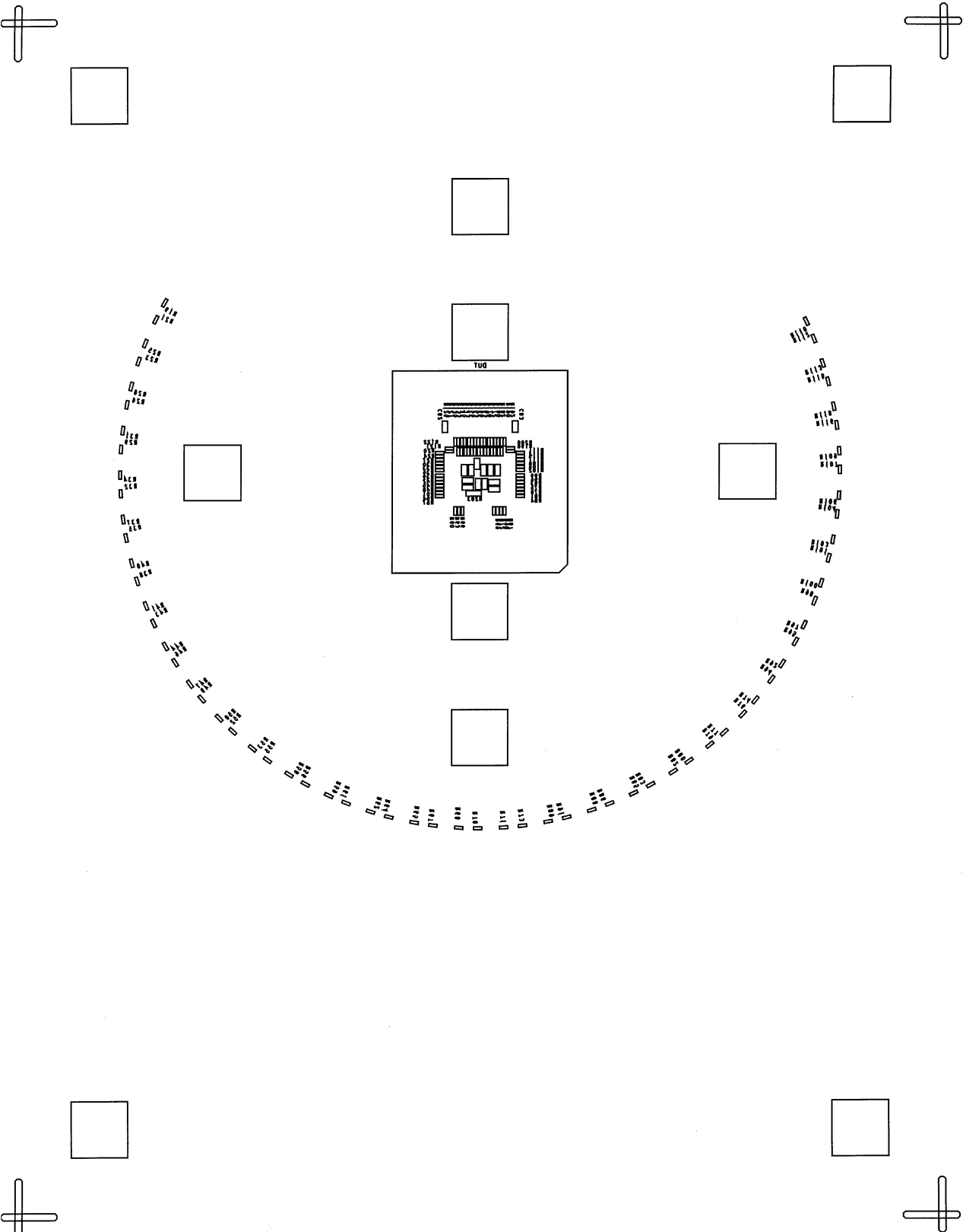
Figure 45. Silkscreen Bottom
