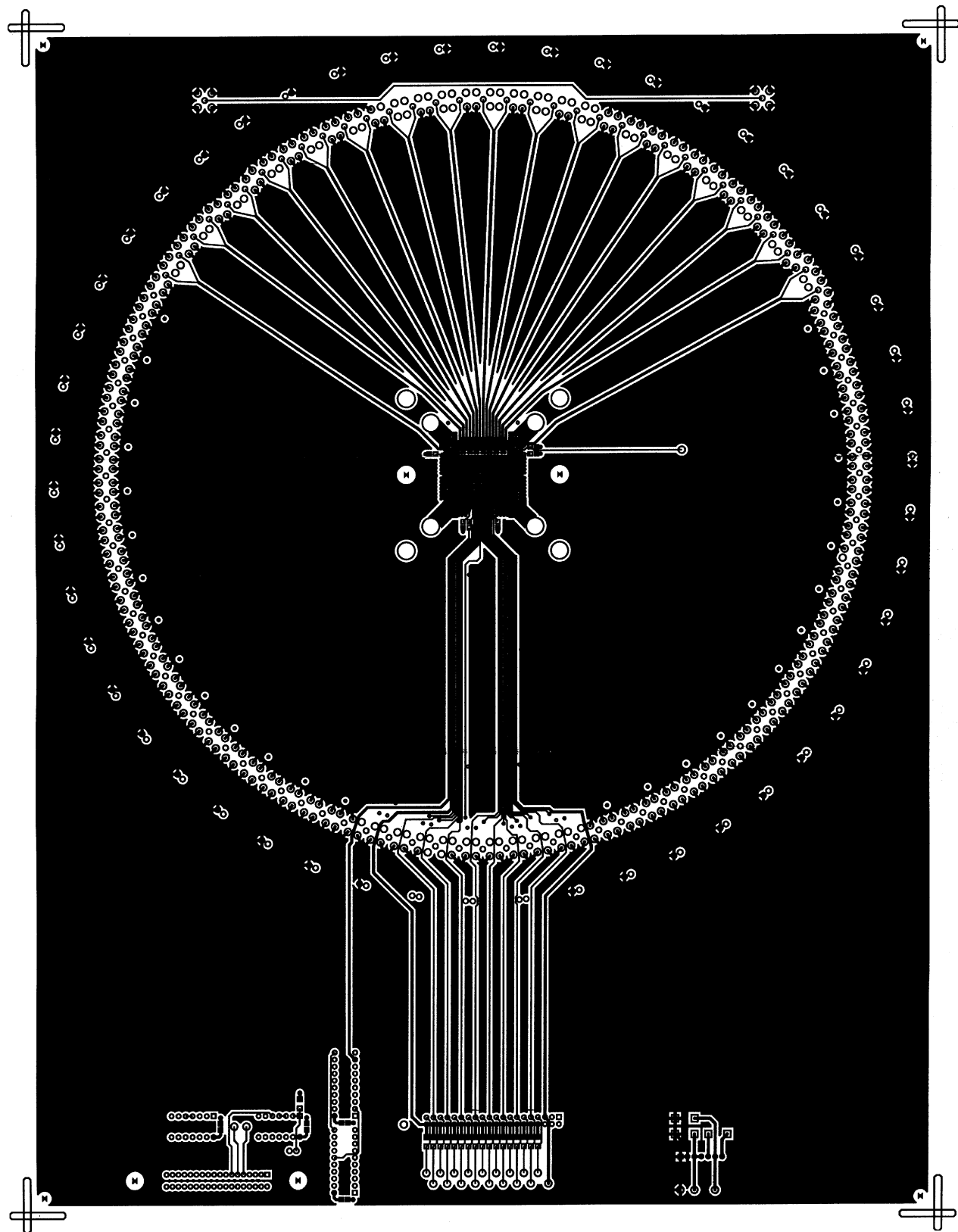
Figure 41. Component Side
