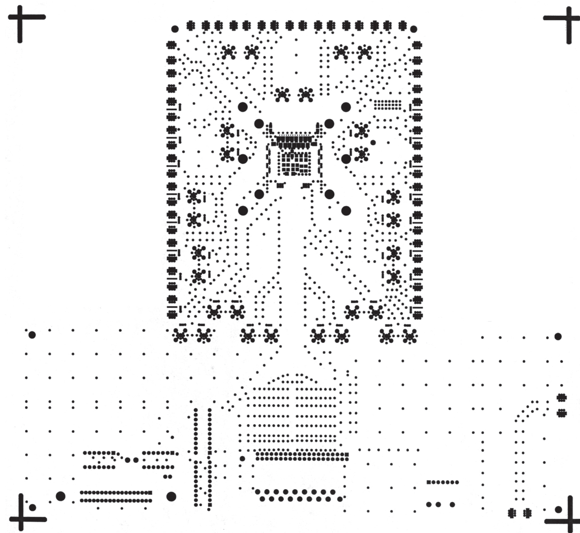
Figure 24. Soldermask Bottom
