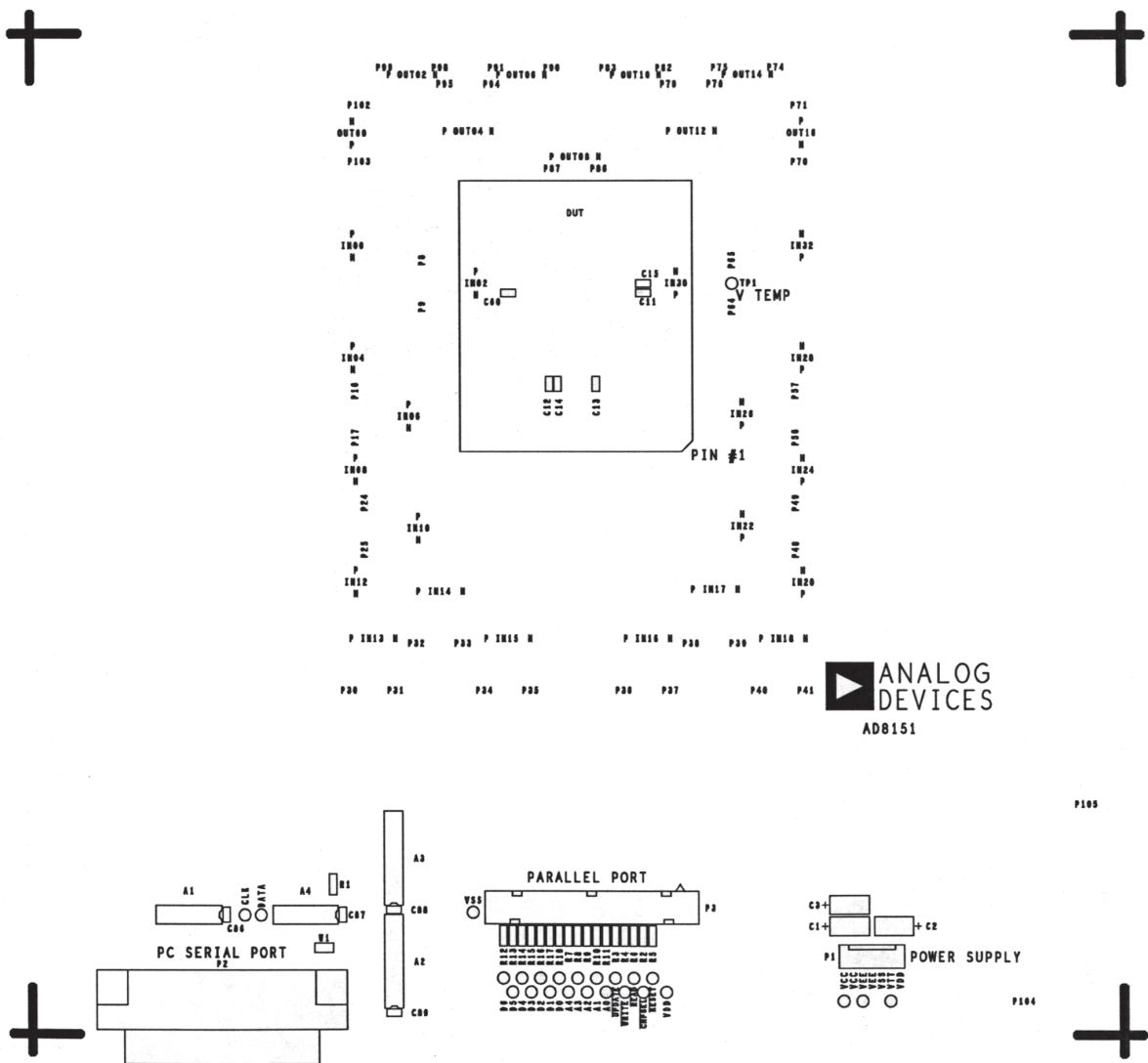
Figure 21. Silkscreen Top
