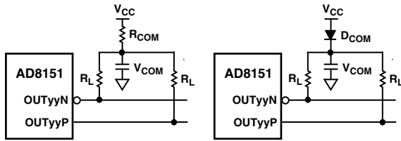
Figure 12. Output Pull-Up Networks: a) ECL 100 k \Omega , b) ECL 10 k \Omega
