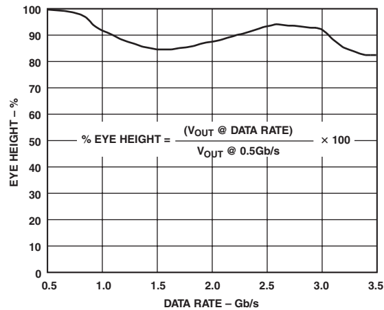
TPC 6. Eye Height vs. Data Rate, PRBS 23
