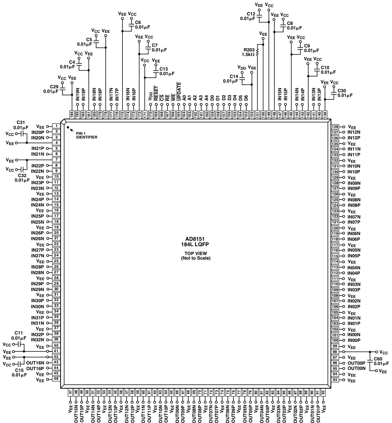
Figure 27. Bypassing Schematic
