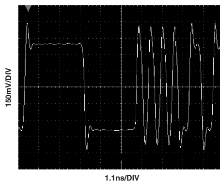
TPC 16. Response, 3.2 Gb/s, 32-Bit Pattern 1111 1111 0000 0000 0101 0101 0011 0011
