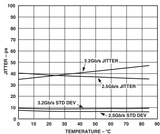
TPC 10. Jitter vs. Temperature, PRBS 23
