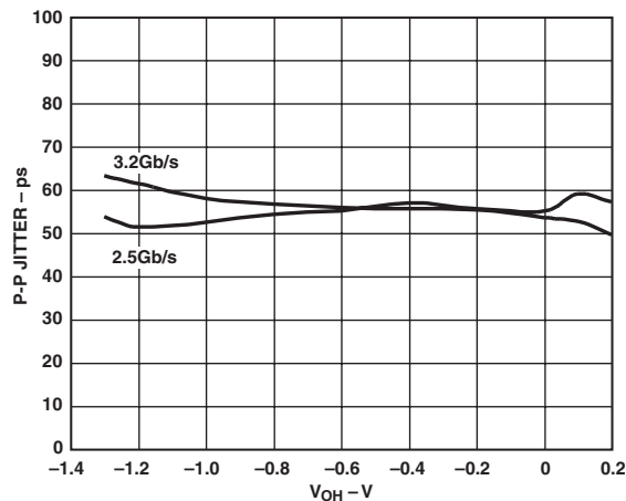
TPC 18. Jitter vs. V_{OH} , PRBS 23, Output Amplitude = 0.4 V Single-Ended
