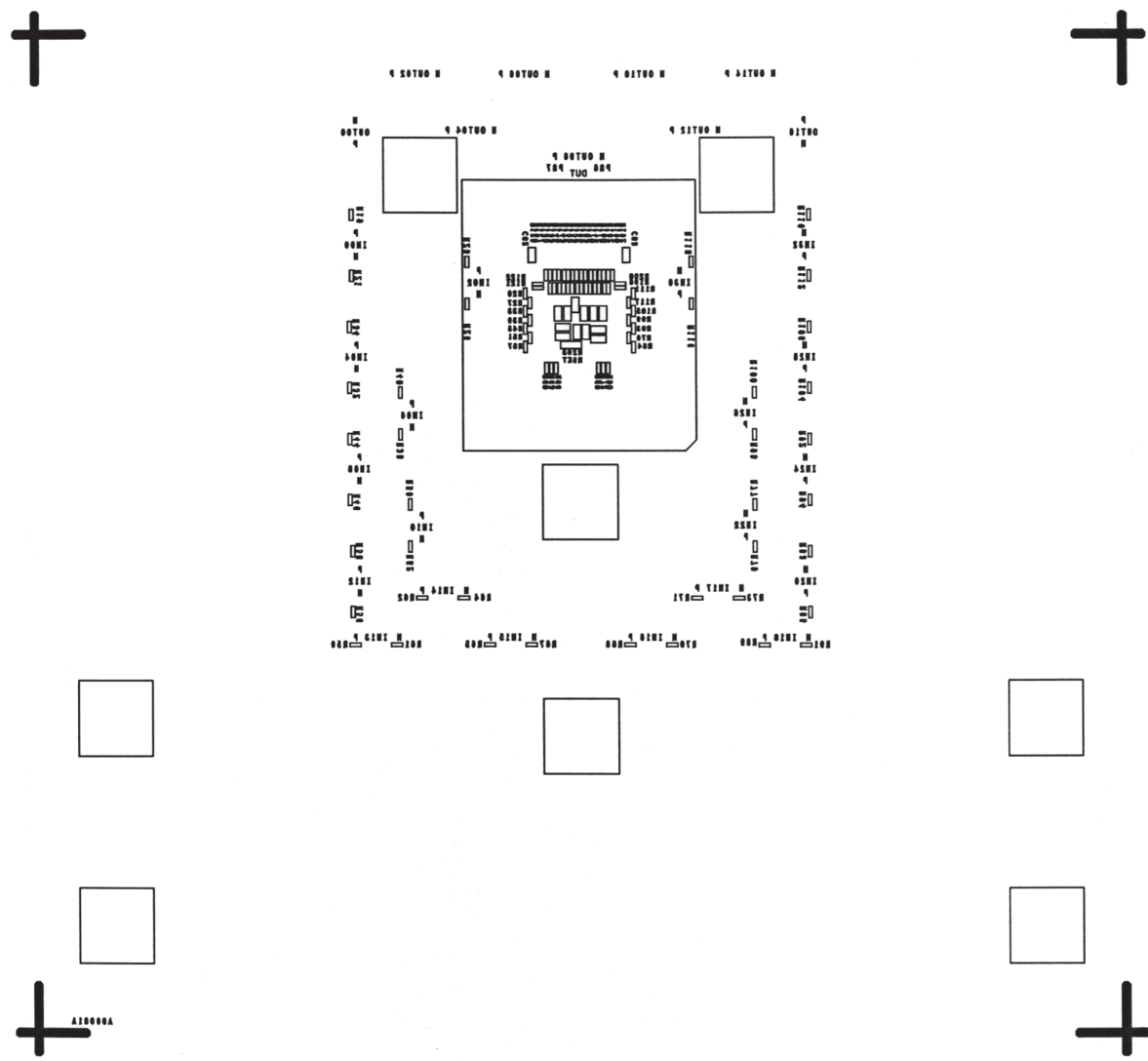
Figure 23. Silkscreen Bottom
