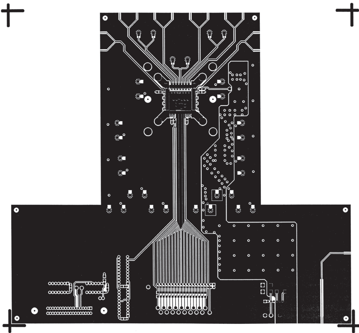
Figure 19. Component Side
