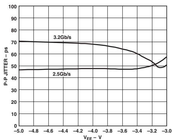
TPC 17. Jitter vs. Supply, PRBS 23
