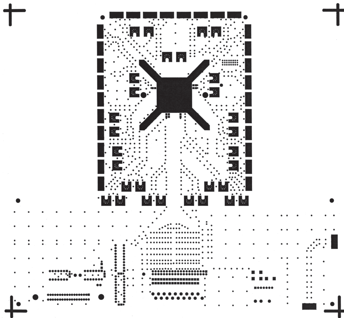
Figure 22. Soldermask Top
