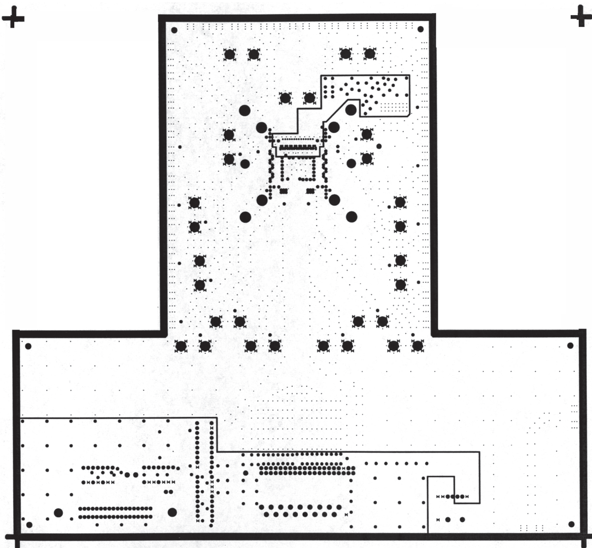
Figure 26. INT2 ( V_{CC} )
