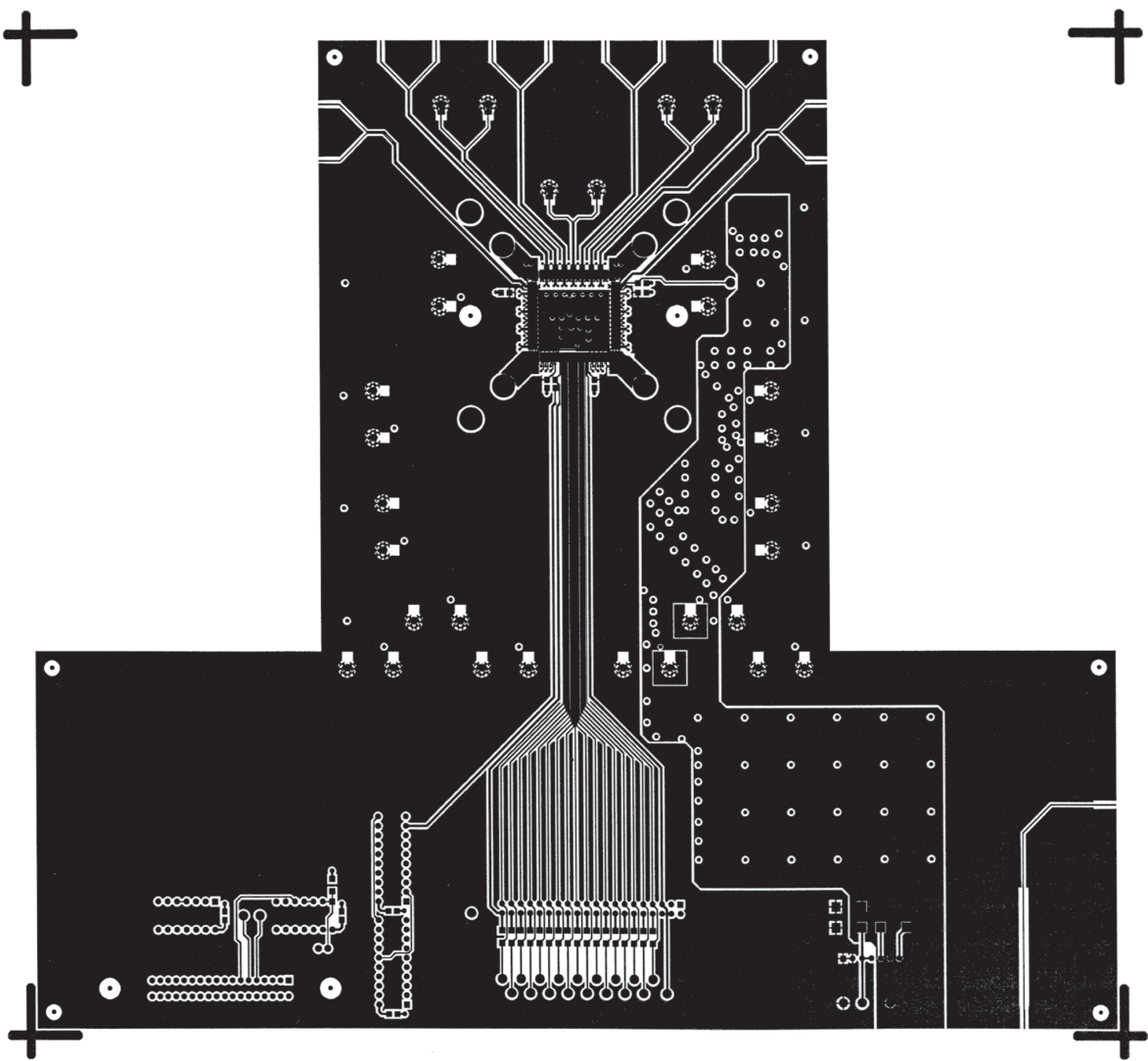
Figure 19. Component Side
