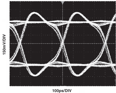
TPC 1. Eye Pattern 2.5 Gb/s, PRBS 23
