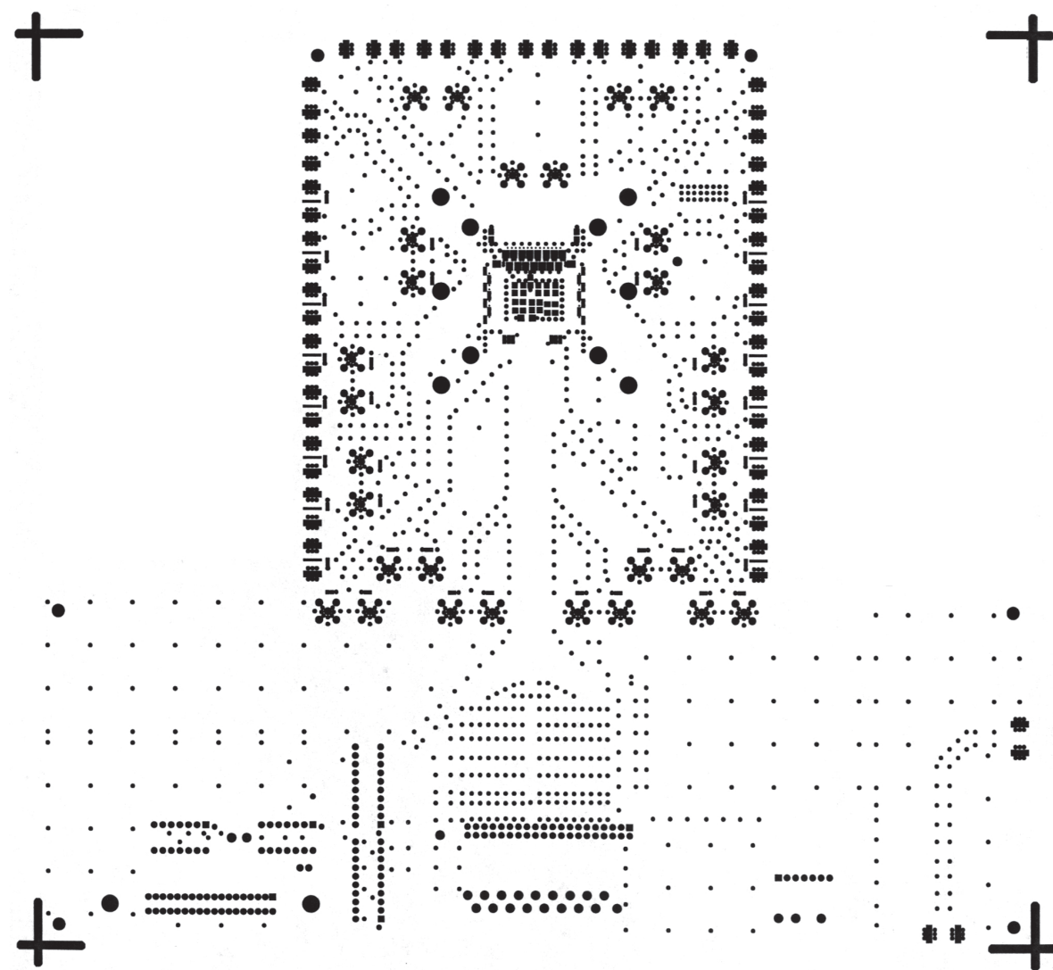
Figure 24. Soldermask Bottom
