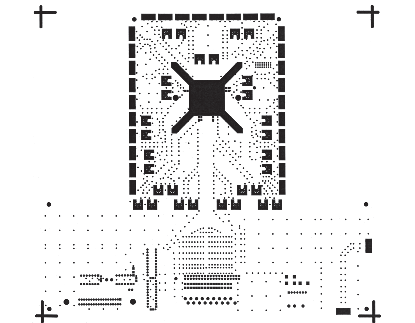
Figure 22. Soldermask Top
