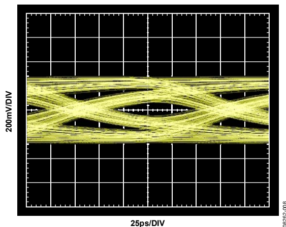
Figure 8. 6.5 Gbps Input Eye, 20 Inch FR4 Input Channel (TP2 from Figure 7)
