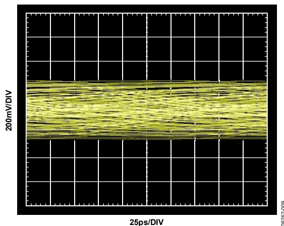
Figure 9. 6.5 Gbps Input Eye, 40 Inch FR4 Input Channel (TP2 from Figure 7)
