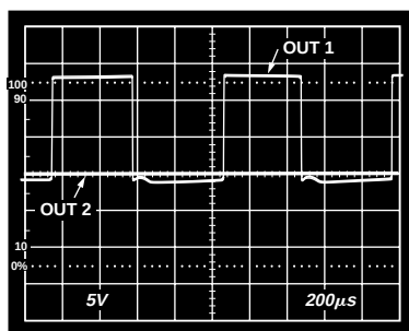
Figure 46. OUT2 Shorted to Ground, Square Wave Is OUT1, R_F = 1\text{ k}\Omega , R_G = 222\text{ }\Omega
