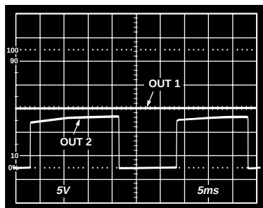
Figure 47. OUT1 Shorted to Ground, Square Wave Is OUT2, R_F = 1\text{ k}\Omega , R_G = 222\text{ }\Omega
