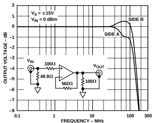
Figure 27. -3 dB Bandwidth vs. Frequency, G = +1
