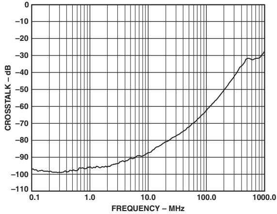
TPC 8. AD8186 Adjacent Channel Crosstalk* vs. Frequency
