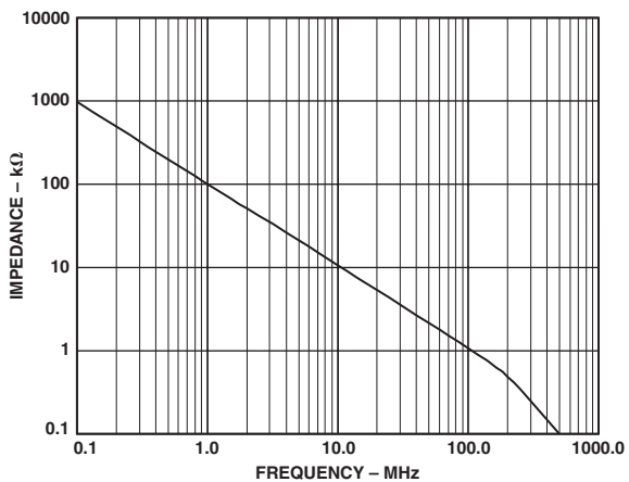
TPC 21. AD8186 Disabled Output Impedance vs. Frequency
