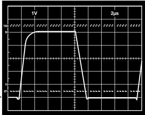
Figure 37. V_S = 5\text{ V}, 0\text{ V} ; Unity-Gain Follower Response to 0 V to 5 V Step
