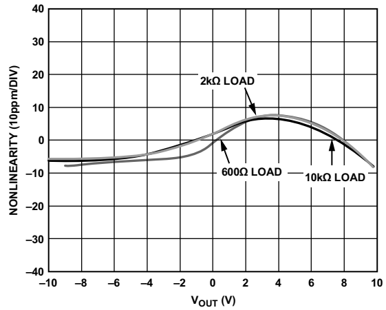
Figure 24. Gain Nonlinearity, G = 100
