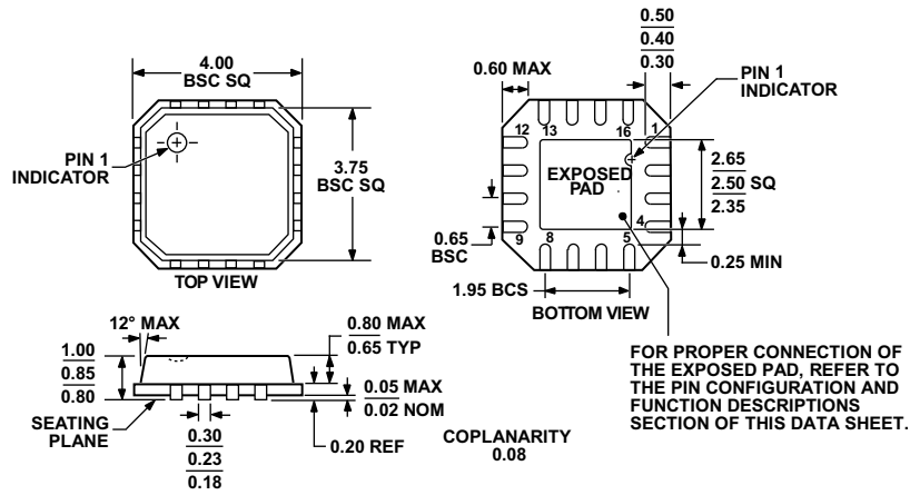
Figure 54. 16-Lead Lead Frame Chip Scale Package [LFCSP_VQ] 4 mm × 4 mm Body, Very Thin Quad (CP-16-13) Dimensions are shown in millimeters
