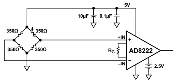
Figure 52. Precision Strain Gauge
