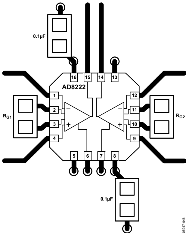
Figure 46. Example Layout
