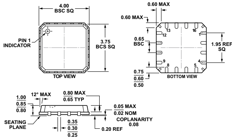
Figure 55. 16-Lead Lead Frame Chip Scale Package [LFCSP_VQ] 4 mm × 4 mm Body, Very Thin Quad, with Hidden Paddle CP-16-19 Dimensions shown in millimeters
