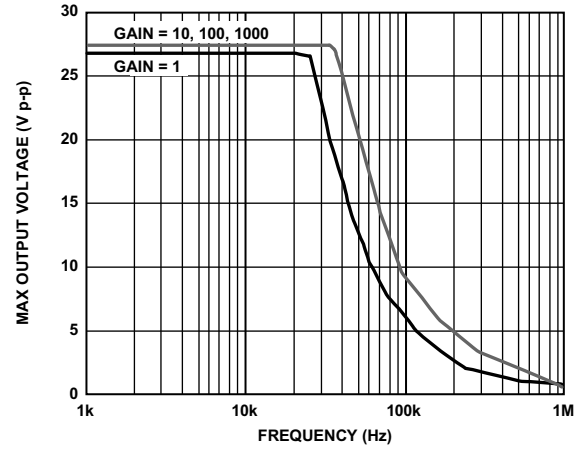
Figure 30. Large Signal Frequency Response
