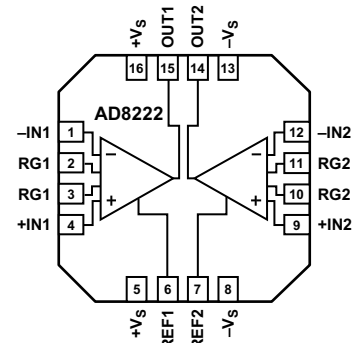
Figure 1. 4 mm × 4 mm LFCSP
