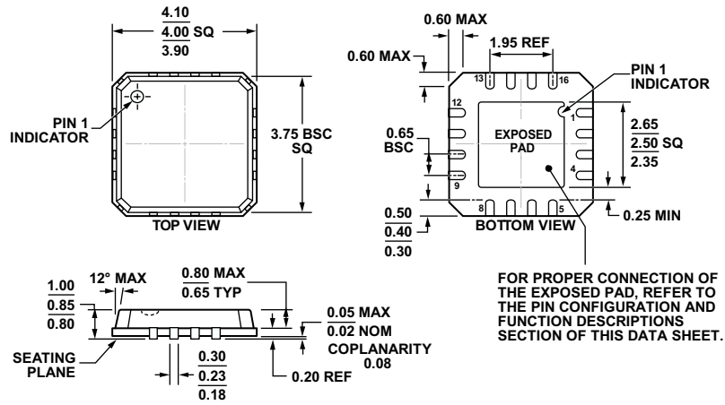
COMPLIANT TO JEDEC STANDARDS MO-220-VGGC Figure 67. 16-Lead Lead Frame Chip Scale Package [LFCSP_VQ] 4 mm × 4 mm Body, Very Thin Quad (CP-16-13) Dimensions are shown in millimeters
