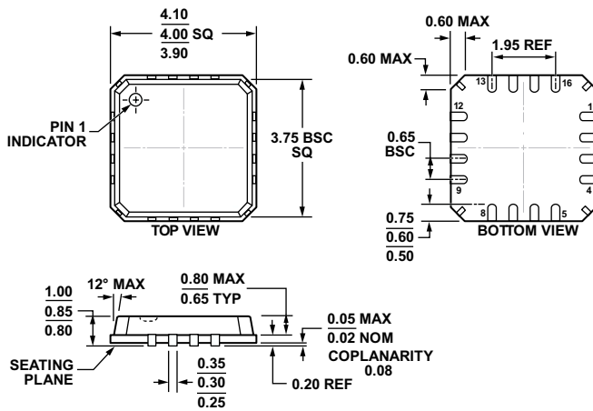
COMPLIANT TO JEDEC STANDARDS MO-263-VBBC Figure 68. 16-Lead Lead Frame Chip Scale Package [LFCSP_VQ] 4 mm × 4 mm Body, Very Thin Quad, with Hidden Paddle (CP-16-19) Dimensions shown in millimeters
