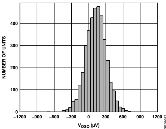
Figure 6. Typical Distribution of Output Offset Voltage
