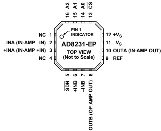
Figure 2. Pin Configuration
