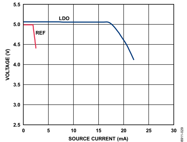
Figure 26. LDO and Reference Voltage vs. LDO Source Current, Stack Voltage = 7.5 V
