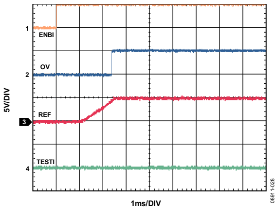
Figure 41. Start-Up Time
