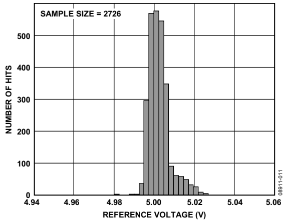
Figure 11. Reference Voltage
