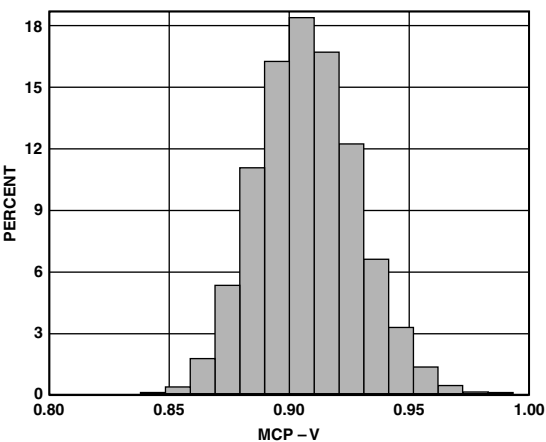
TPC 16. Center Point of Magnitude Output (MCP) Distribution Frequencies 900 MHz, 17,000 Units
