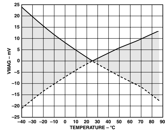
TPC 15. Change in Center Point of Magnitude Output (MCP) vs. Temperature, Three Sigma to Either Side of Mean Frequencies 1900 MHz
