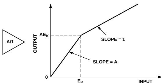
Figure 21. The A/1 Amplifier Function
