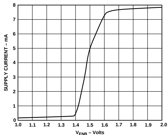
Figure 1. Supply Current vs. V_{ENB} Voltage (5 V)
