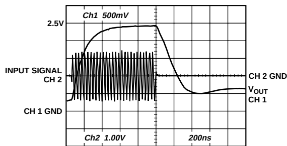
Figure 17. Large Signal Response Time
