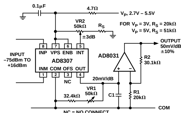
Figure 36. Log Amp with Buffered Output
