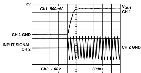
Figure 16. V_{OUT} Rise Time
