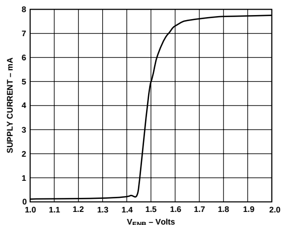
Figure 2. Supply Current vs. V_{ENB} Voltage (3 V)
