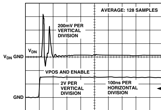
TPC 23. Power-On Response, V_{DN} , Controller Mode with VSET Held Low
