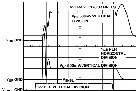
TPC 13. ENBL Response Time
