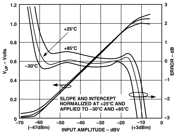
TPC 3. V_{UP} and Log Conformance vs. Input Amplitude at 0.9 GHz; -30^{\circ}\text{C} , +25^{\circ}\text{C} , and +85^{\circ}\text{C}
