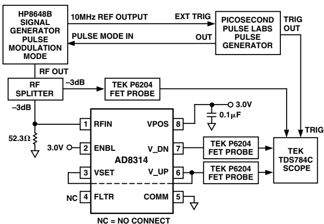
TPC 17. Test Setup for Pulse Response
