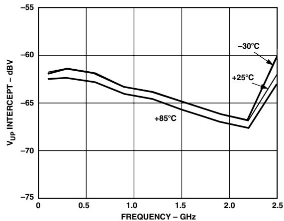
TPC 10. V_{UP} Intercept vs. Frequency: -30^{\circ}\text{C} , +25^{\circ}\text{C} , and +85^{\circ}\text{C}
