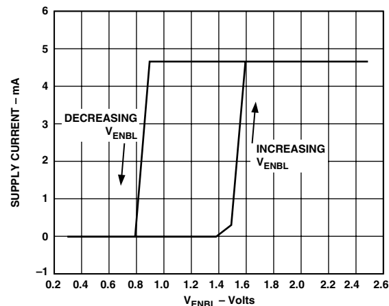
TPC 12. Supply Current vs. ENBL Voltage, V_S = 3\text{ V}
