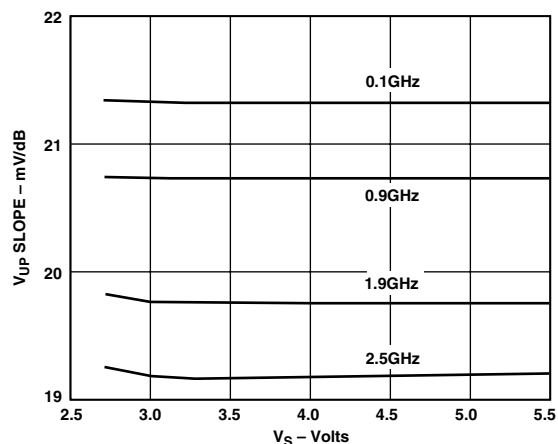
TPC 8. V_{UP} Slope vs. Supply Voltage
