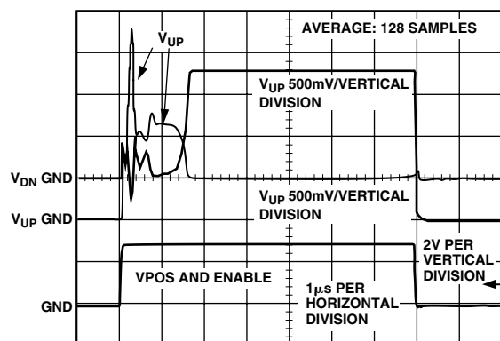
TPC 20. Power-On and Power-Off Response, Measurement Mode
