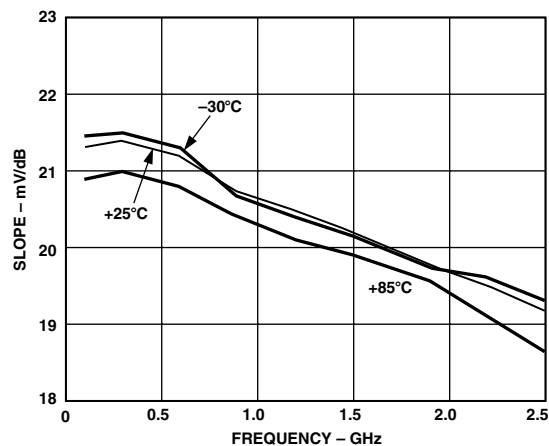
TPC 7. Slope vs. Frequency; -30^{\circ}\text{C} , +25^{\circ}\text{C} , and +85^{\circ}\text{C}
