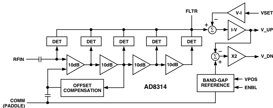
Figure 1. Block Schematic
